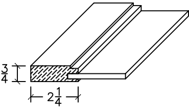
5-piece shaker door front with double step inside rail profile
